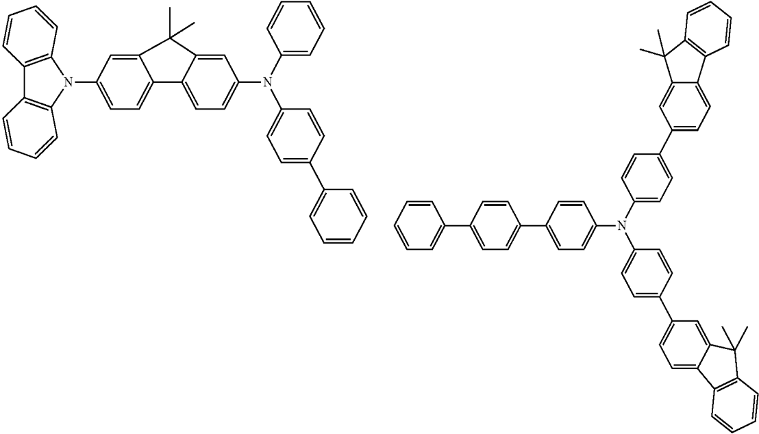
HT19
