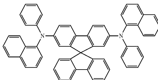
Spiro-NPB
