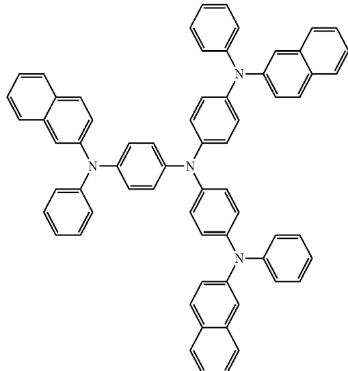
2-TNATA
