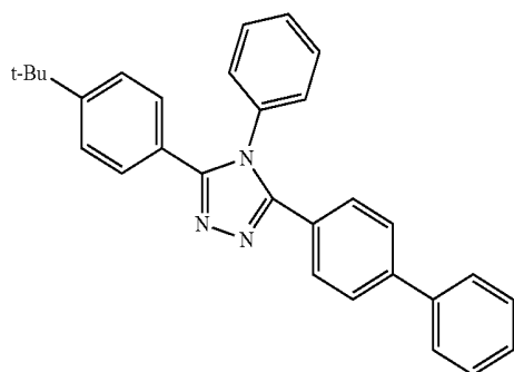
TAZ
